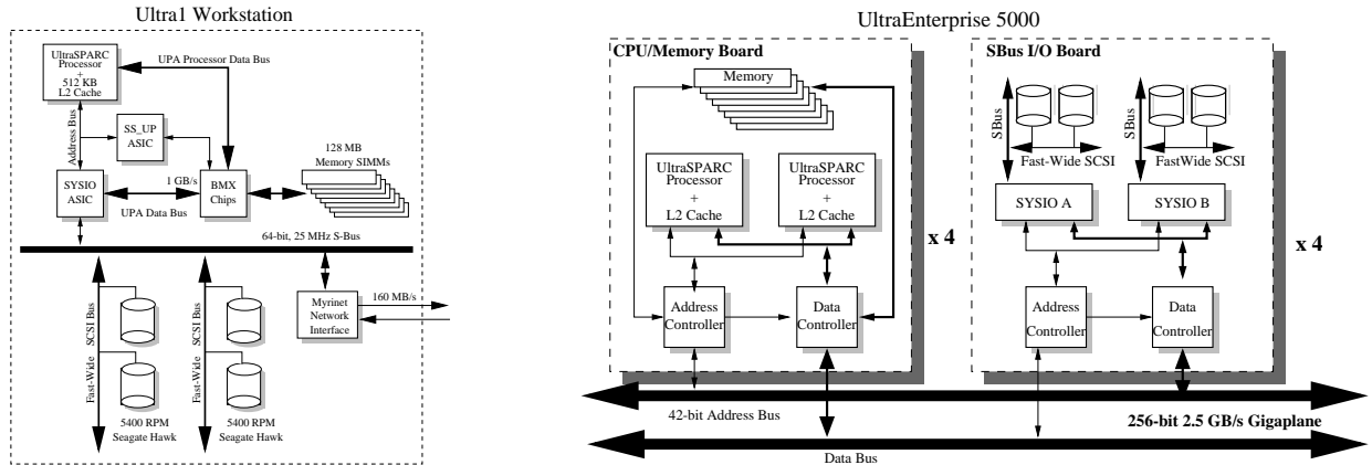
Figure 1: Hardware Diagram. This figure depicts the internals of an Ultra 1 workstation and the Ultra Enterprise 5000. Workstation: Inside the workstation on the left, the BMX crossbar chips and SS_UP ASIC controller provide switched-based access to memory. SMP: On the right is the Enterprise 5000. Each CPU board houses two CPUs, which share an address and a data bus. Each I/O board consists of two S-Bus I/O busses. All boards are connected to the main memory interconnect (GigaPlane). Though memory is physically distributed, access time is uniform.
